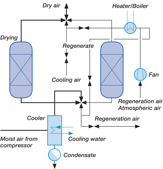
Figure 1 Compressed-air dryer with purgeless regeneration
