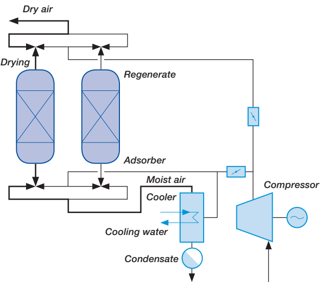
Figure 2 Compressed air dryer with Heat-of-Compression (HOC)
